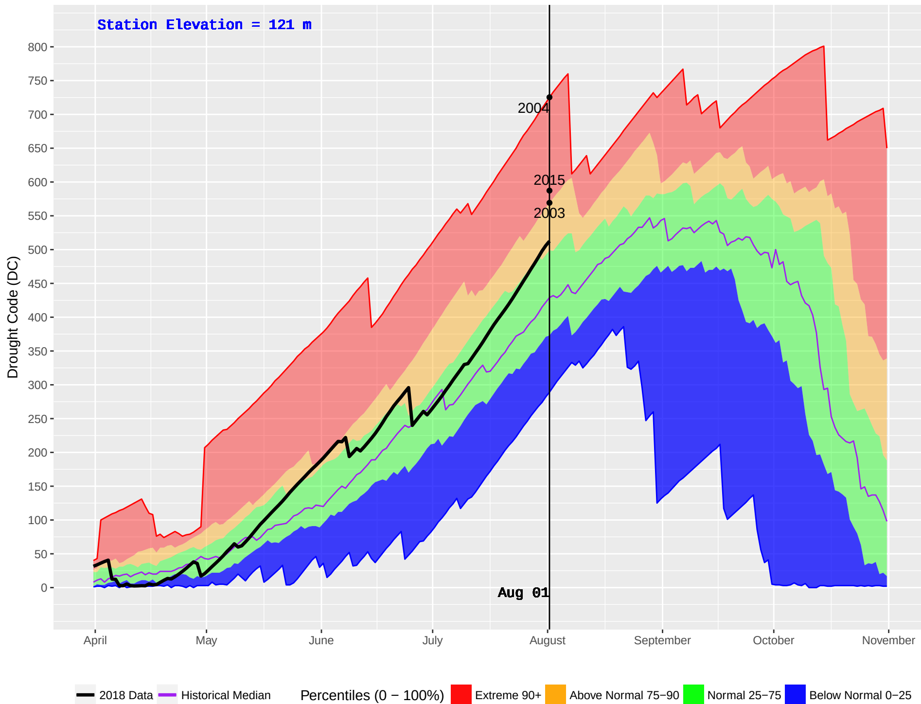
BOWSER (56) : Historical (1985–2016) and Current (2018) Daily Drought Code (DC)
