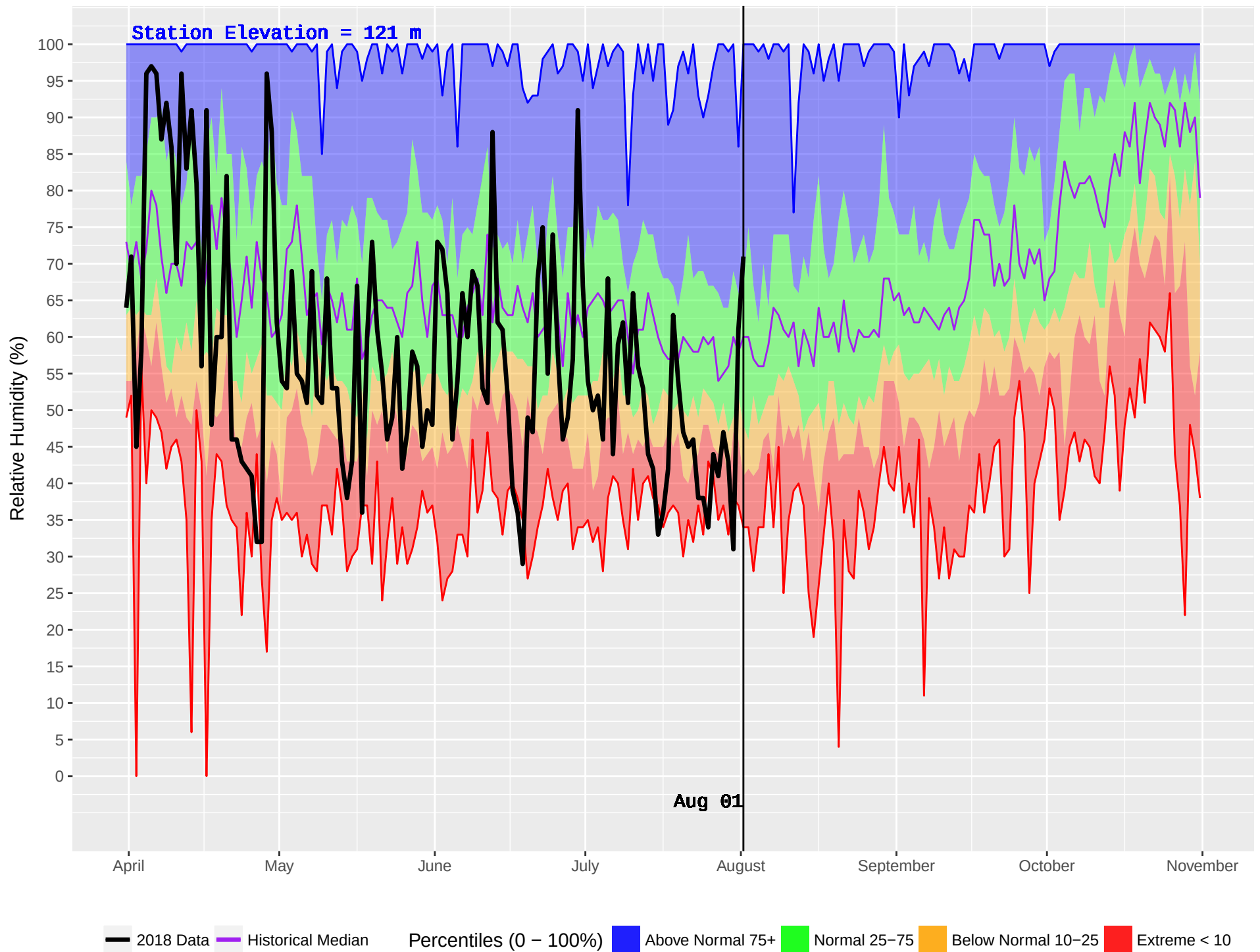
BOWSER (56) : Historical (1985–2016) and Current (2018) Daily Relative Humidity
